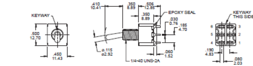
Part No. Shown : 1MD1T1B1M1QE
